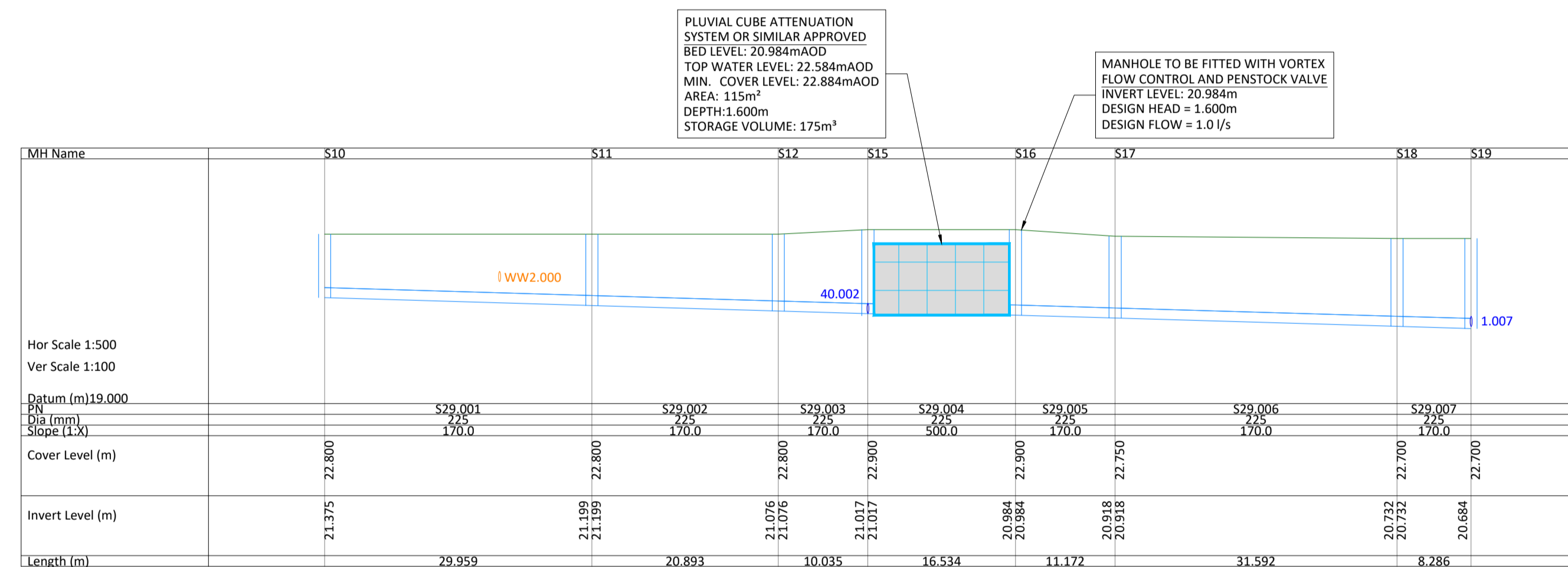
SURFACE WATER DRAINAGE BRANCH S29.000
