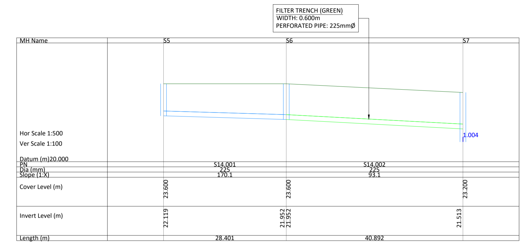
SURFACE WATER DRAINAGE BRANCH S14.000
