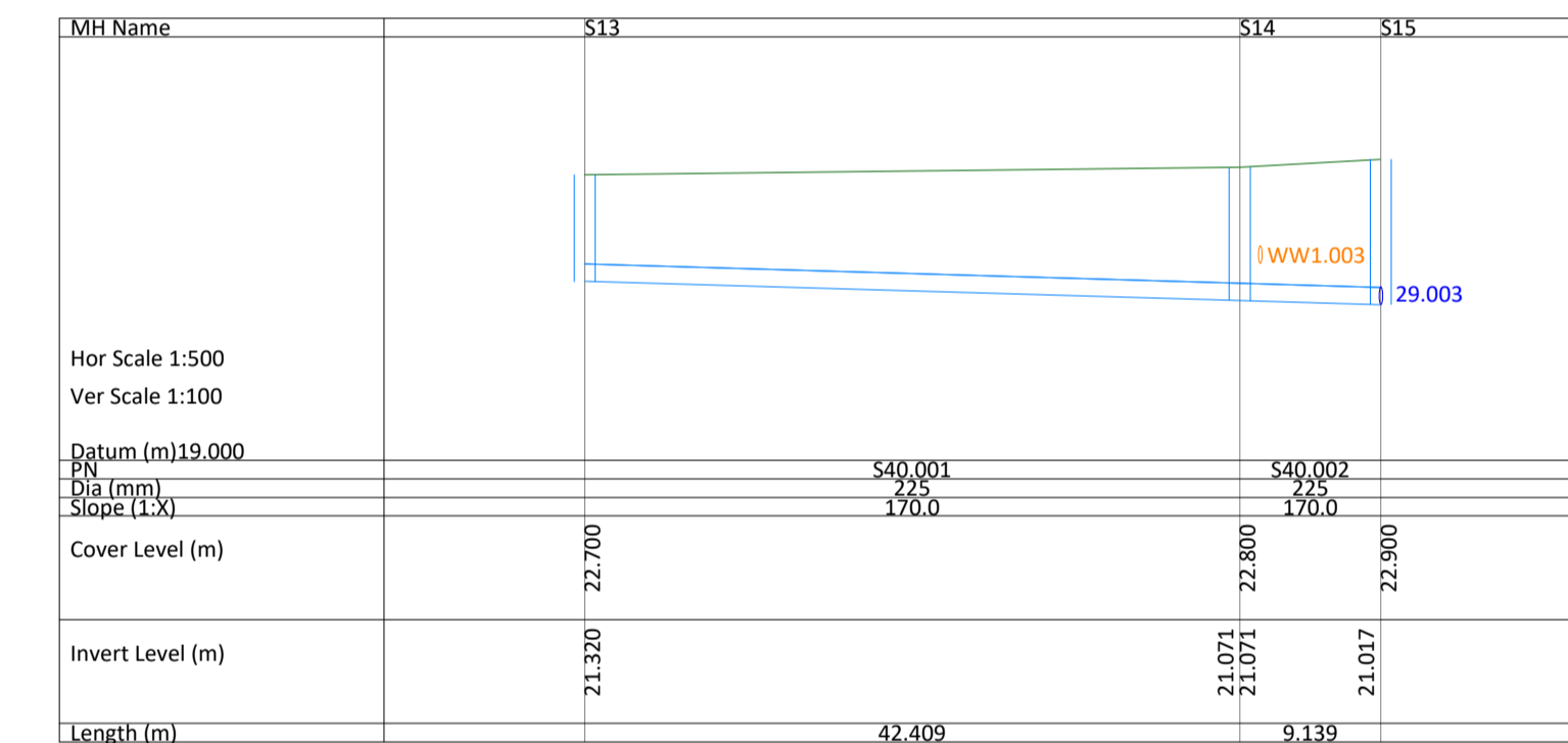
SURFACE WATER DRAINAGE BRANCH S40.000
