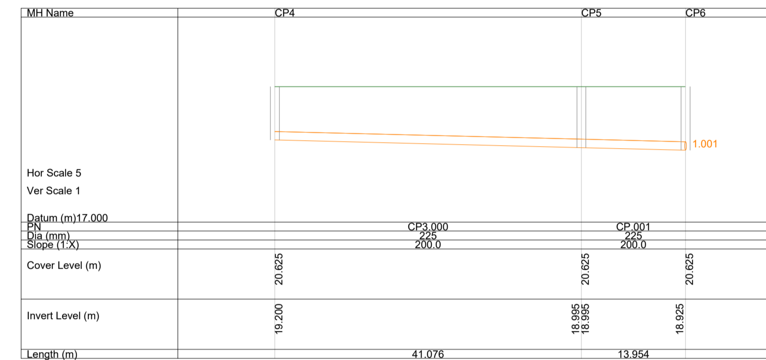
CARPARK DRAINAGE BRANCH CP3.000
