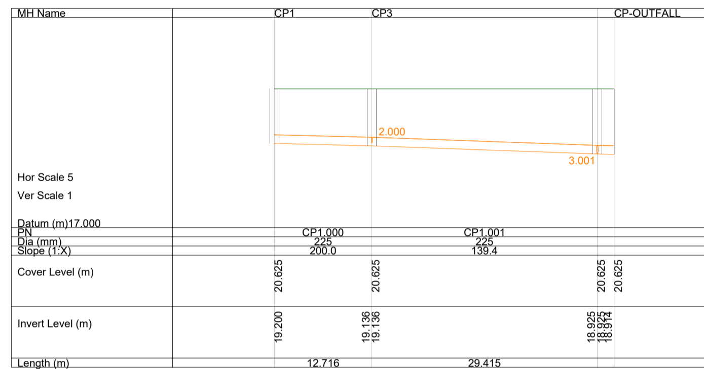
CARPARK DRAINAGE BRANCH CP1.000
