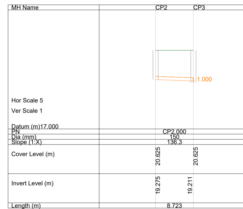
CARPARK DRAINAGE BRANCH CP2.000
