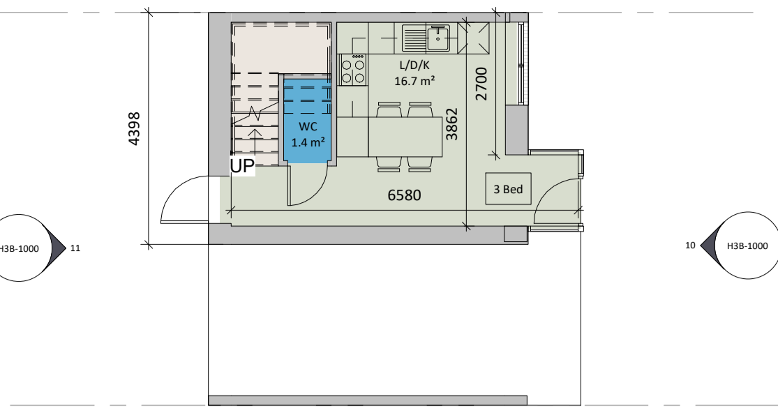
1 Level 00 - Typical Unit 1:100
