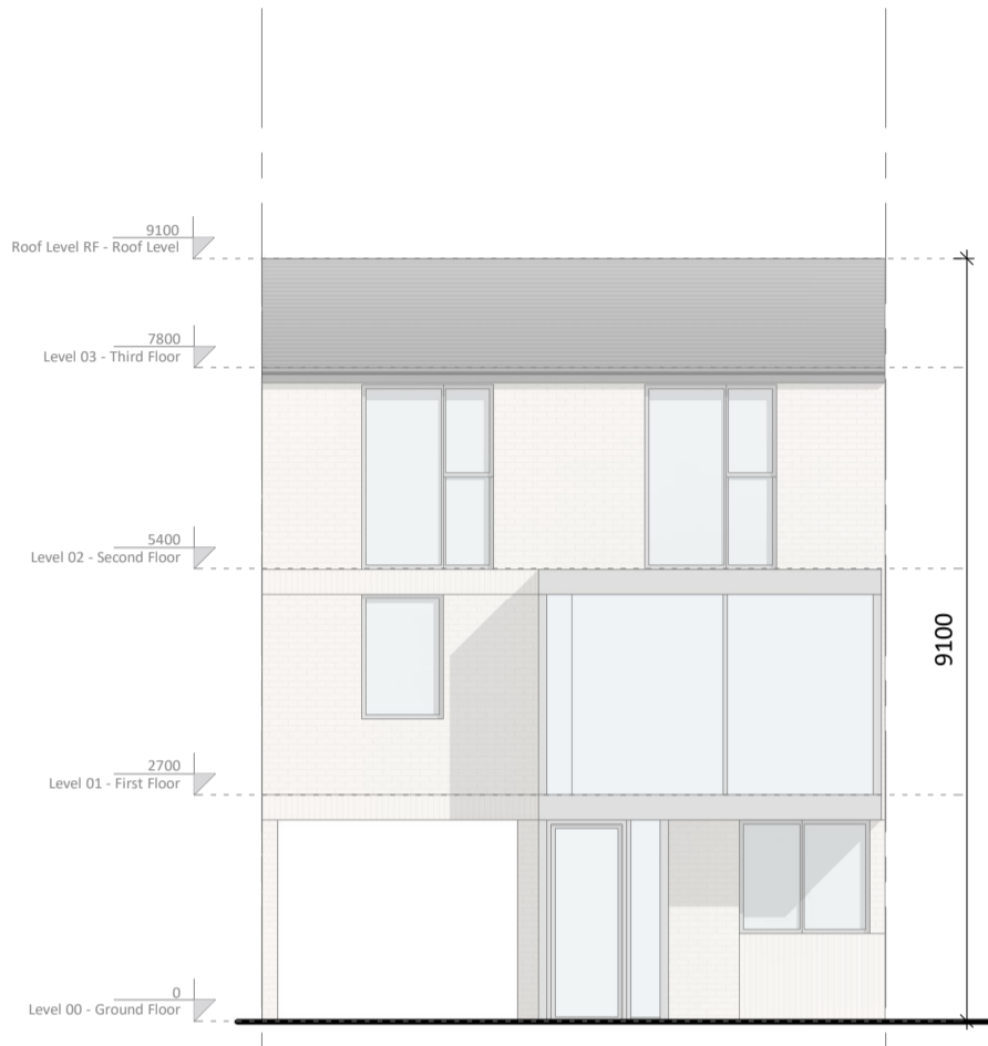
10 Front Elevation 1:100
