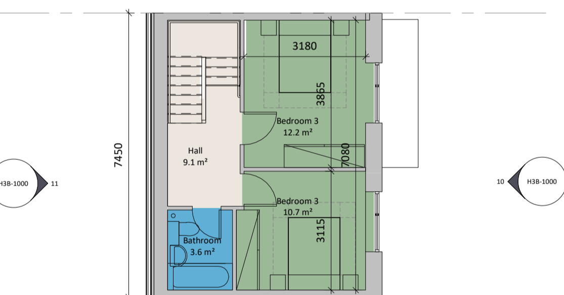
3 Level 02 - Typical Unit 1:100
