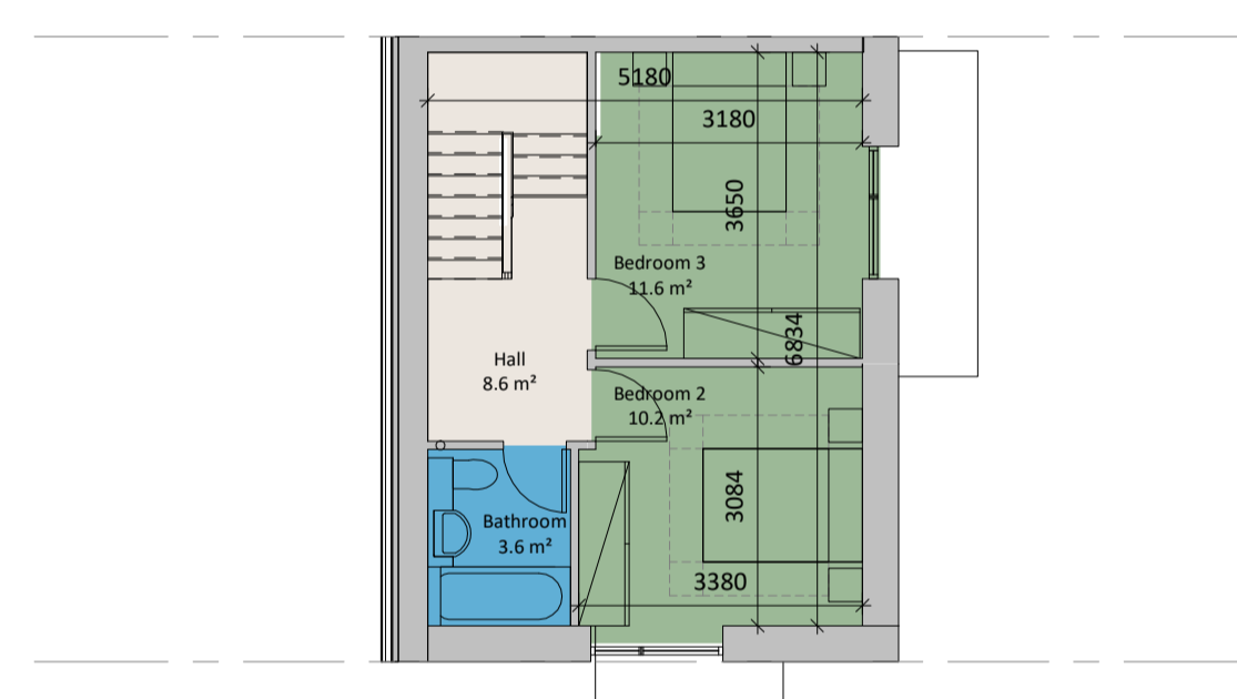
7 Level 02 - End of Terrace 1:100
