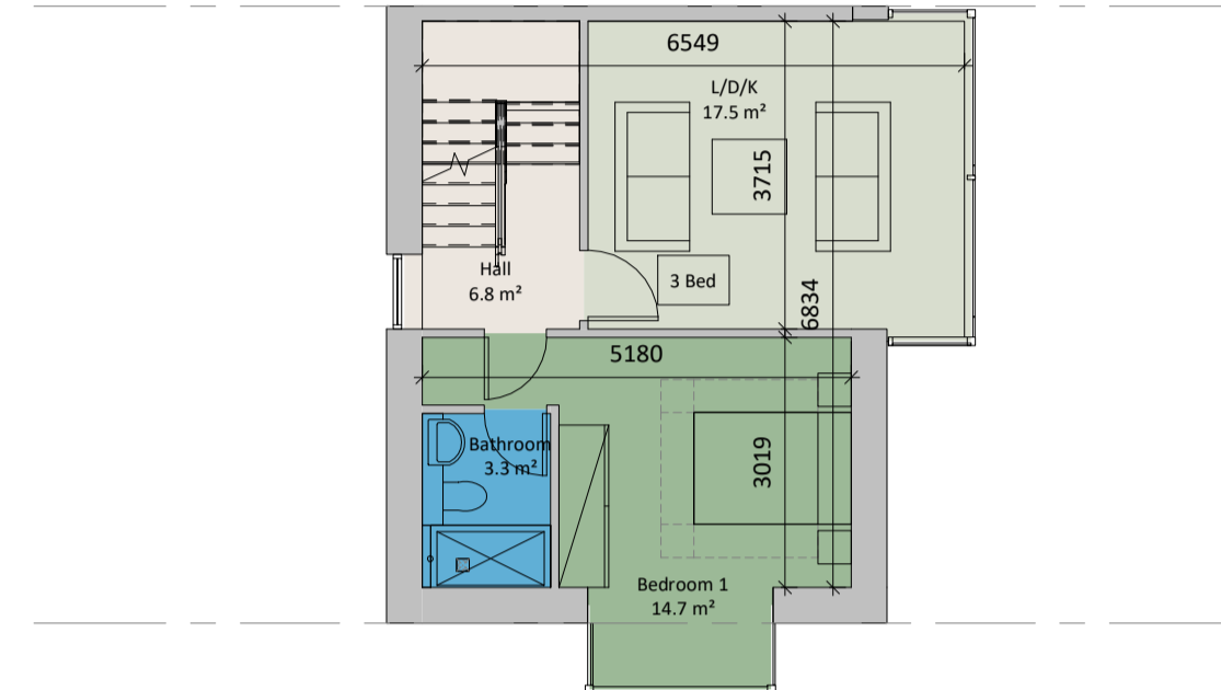
6 Level 01 - End of Terrace 1:100
