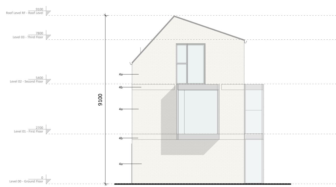
9 End of Terrace - South Elevation 1:100
