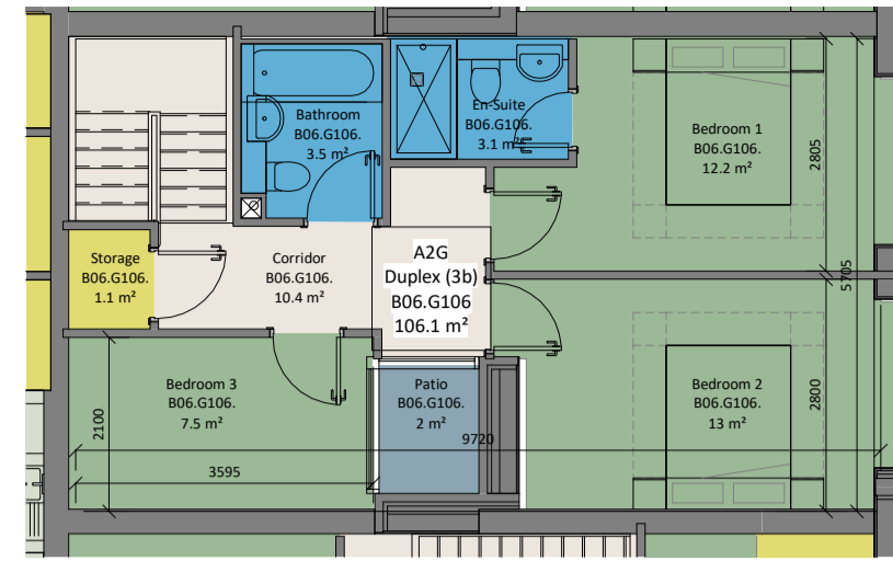
② Unit Type A2G Upper 1:100
