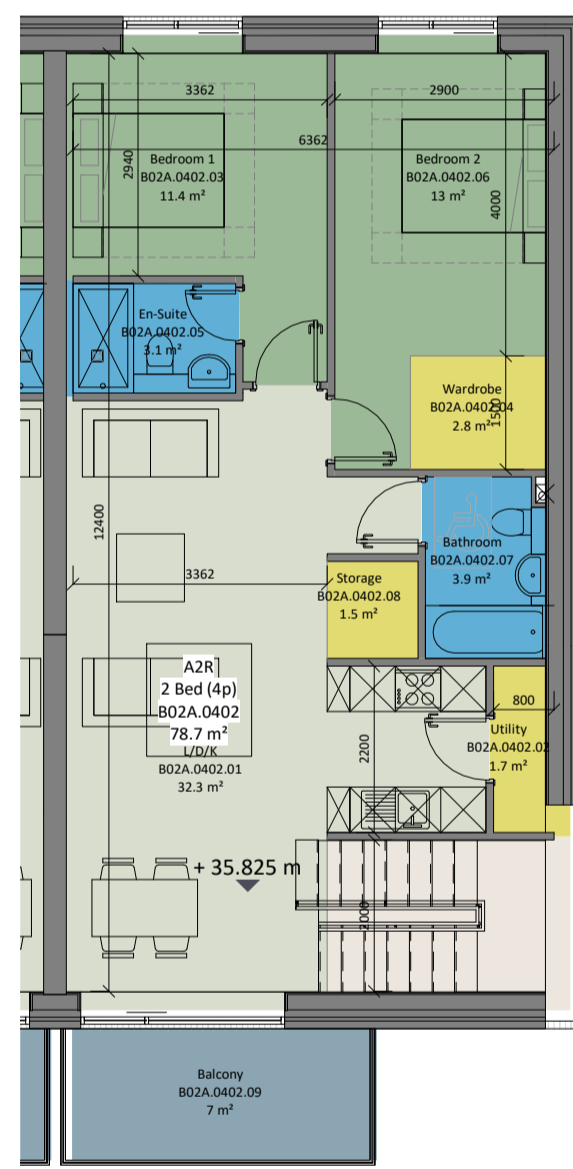
⑤a Unit Type A2R 1:100
