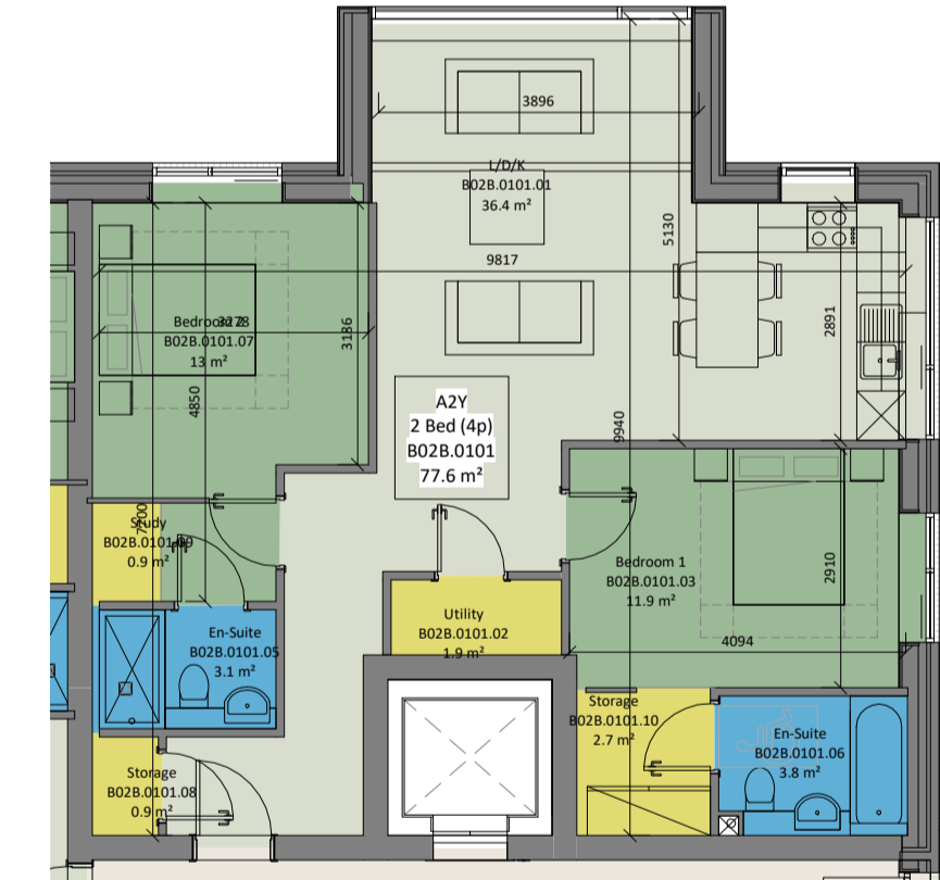
⑨ Unit Type A2Y 1:100
