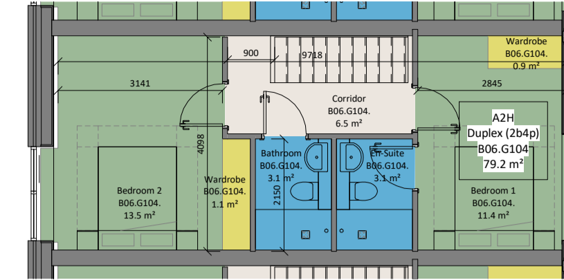
⑮ Unit Type A2H Upper 1:100
