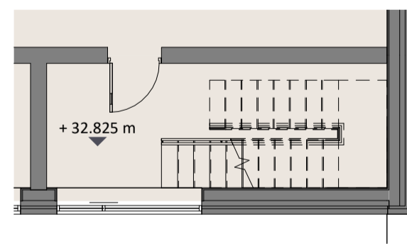
⑤b Unit Type A2R Entrance Level 1:100
