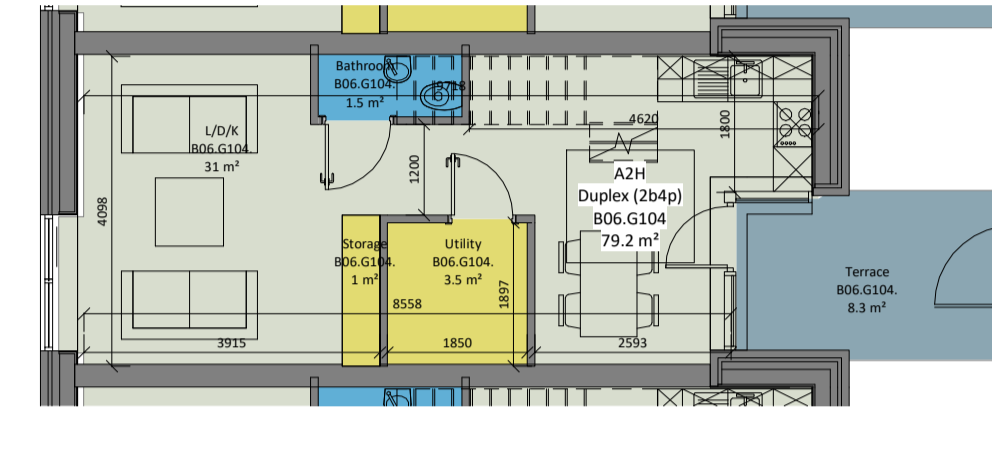
④ Unit Type A2H Lower 1:100
